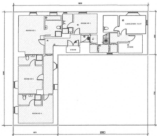
First floor plan as existing scale 1:100
